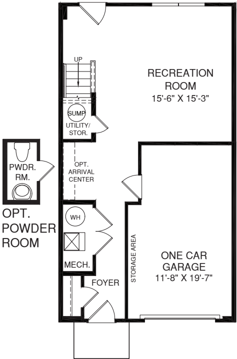
LOWER LEVEL
