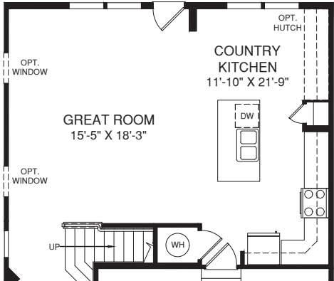
OPT. 2' EXTENSION
