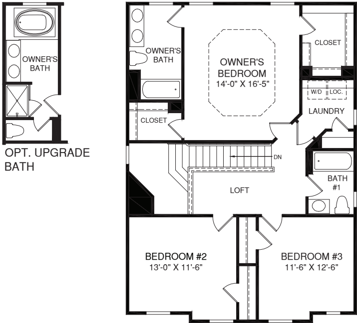
UPPER LEVEL
