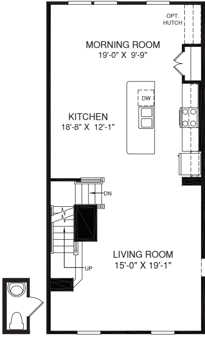
MAIN LEVEL
