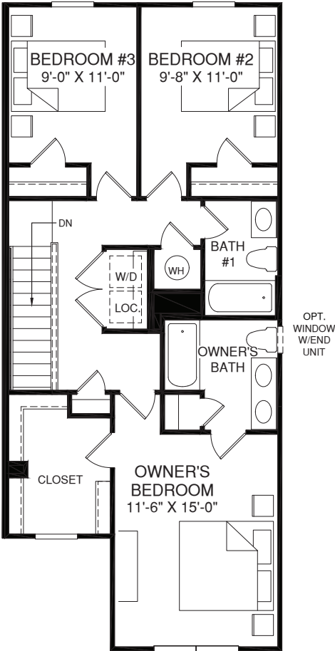
UPPER LEVEL
