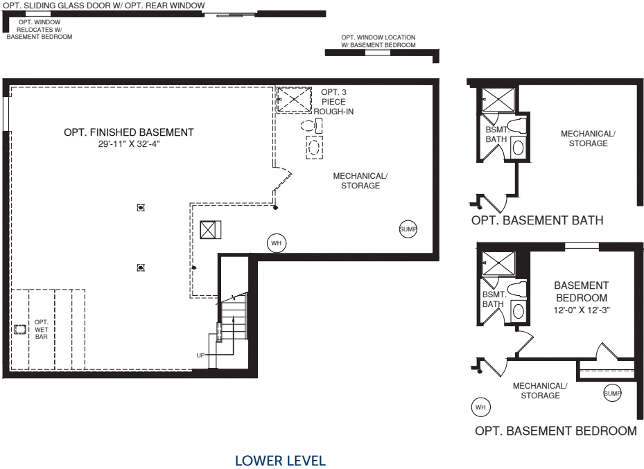
LOWER LEVEL
