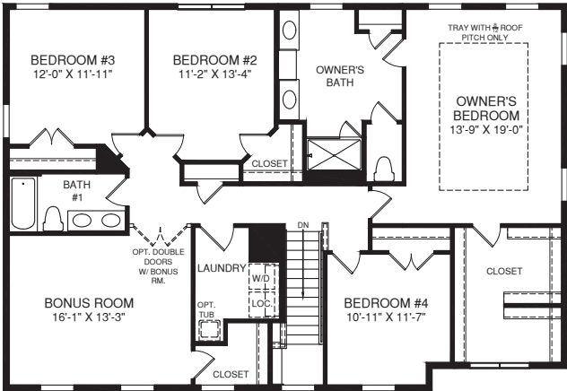
OPT. FOUR BEDROOM W/ BONUS ROOM
